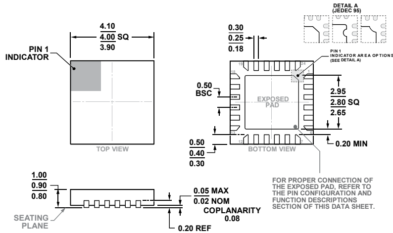
COMPLIANT TO JEDEC STANDARDS MO-220-VGGD-8. Figure 55. 24-Lead Lead Frame Chip Scale Package [LFCSP] 4 mm x 4 mm Body and 0.90 mm Package Height (HCP-24-2) Dimensions shown in millimeters
