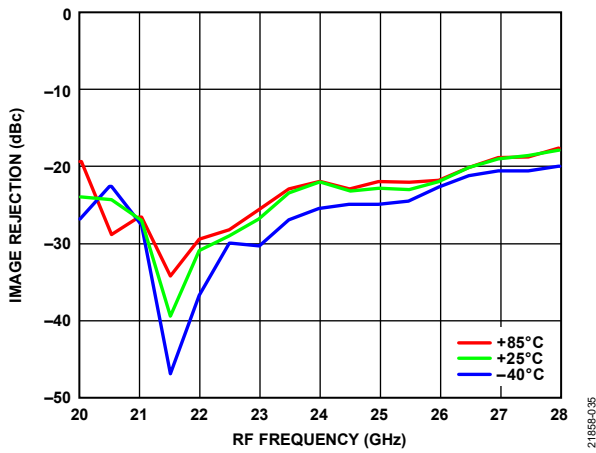
Figure 43. Image Rejection vs. RF Frequency Over Temperature, LO Drive = 6 dBm
