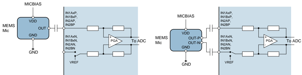
Figure 78 Single-Ended and Differential Analogue Microphone Connections
