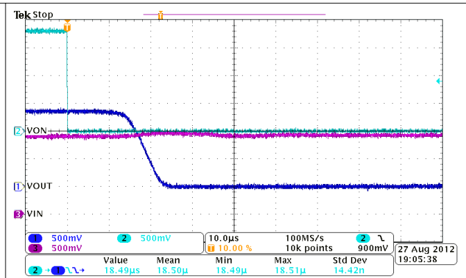
Figure 5-25. Turn-Off Response Time ( V_{IN} = 1.4\text{ V} , C_{IN} = 10\ \mu\text{F} , C_L = 0.1\ \mu\text{F} , R_L = 10\ \Omega )
