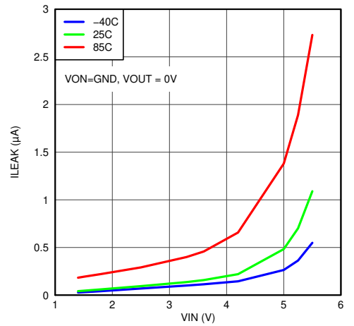
Figure 5-4. I_{IN(\text{leak})} vs V_{IN}
