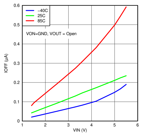
Figure 5-6. I_{IN(\text{off})} vs V_{IN}
