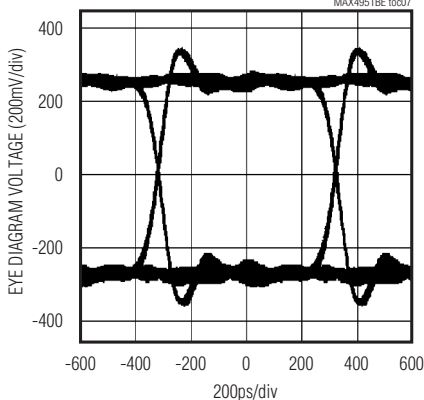
V_{IN} = 220\text{mVp-p} , 1.5Gbps, PA = 1, PB = 1
