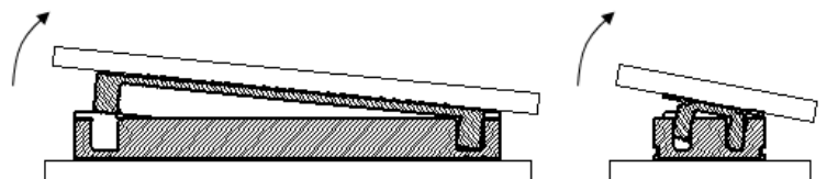
× 図-5 こじり抜去 (Not Good) Figure-5 Un-mating with twisting the connector at an angle
