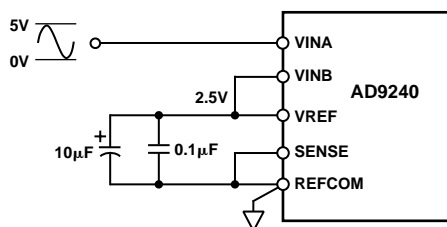
Figure 40. Internal Reference—5 V p-p Input Span, V_{\text{CM}} = 2.5 \text{ V}
