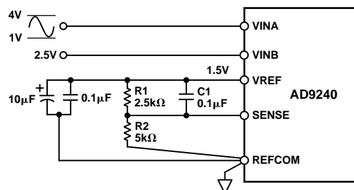
Figure 41. Resistor Programmable Reference (3 V p-p Input Span, V_{\text{CM}} = 2.5 \text{ V} )
