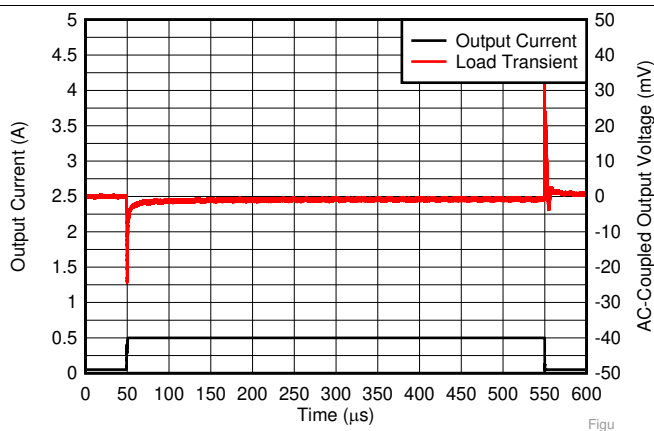
V_{IN} = 1.4\text{ V} , I_{OUT} = 50\text{ mA to } 500\text{ mA to } 50\text{ mA at } 1\text{ A}/\mu\text{s} , C_{OUT} = 10\ \mu\text{F} , V_{PG} = V_{OUT}
