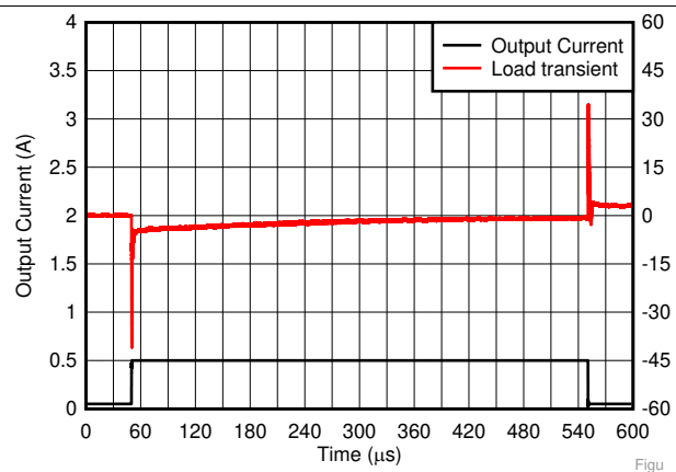
V_{IN} = 5.5\text{ V} , I_{OUT} = 50\text{ mA to } 500\text{ mA to } 50\text{ mA at } 1\text{ A}/\mu\text{s} , C_{OUT} = 10\ \mu\text{F} , V_{PG} = V_{OUT}
