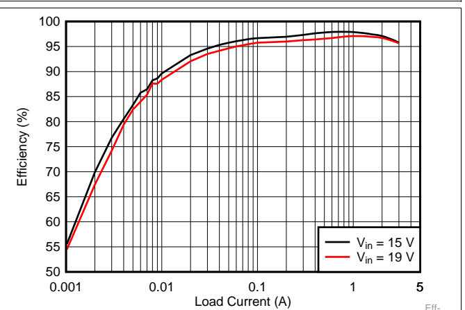
Figure 12. V_{OUT}=3.3\text{ V} Efficiency, L=4.7\ \mu\text{H}
