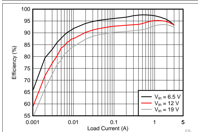
Figure 11. V_{OUT}=1.05\text{ V} Efficiency, L=1.5\ \mu\text{H}
