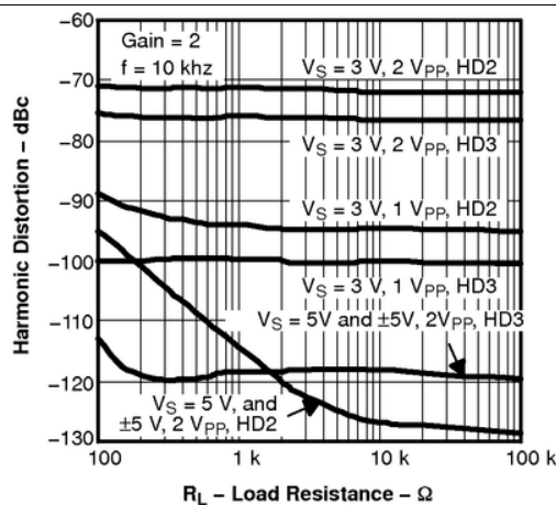
Figure 44. Harmonic Distortion vs Load Resistance
