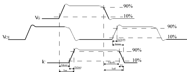
Figure 30. Switching waveform
