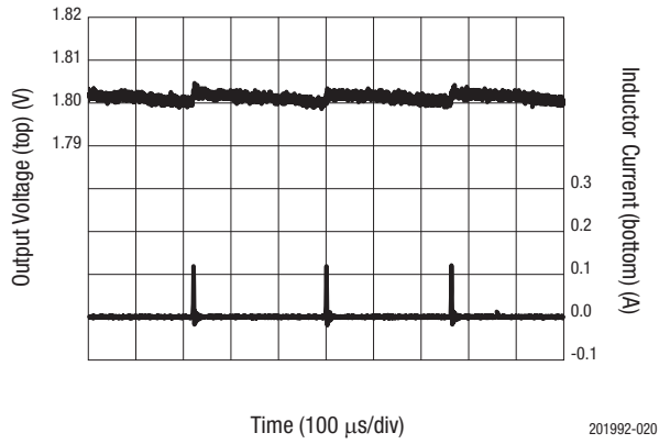
Figure 20. Output Ripple (VIN = 3.6 V, VOUT = 1.8 V, IOUT = 0 A, L = 2.2 μH)
