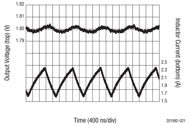
Figure 21. Output Ripple (VIN = 3.6 V, VOUT = 1.8 V, IOUT = 2 A, L = 2.2 μH)
