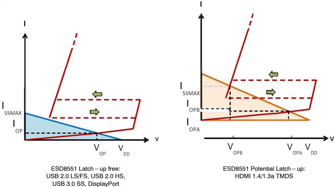
Figure 6. Example Load Lines for Latch-up Free Applications and Applications with the Potential for Latch-up
