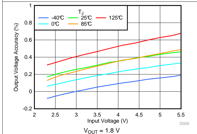
Figure 27. Output Accuracy V_{IN} and Temperature
