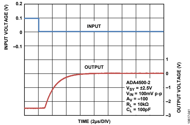
Figure 44. Negative Overload Recovery, V_{SY} = \pm 2.5V
