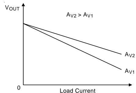
Figure 5. Error Amplifier Gain ( A_v ) Influence on V_{OUT}
