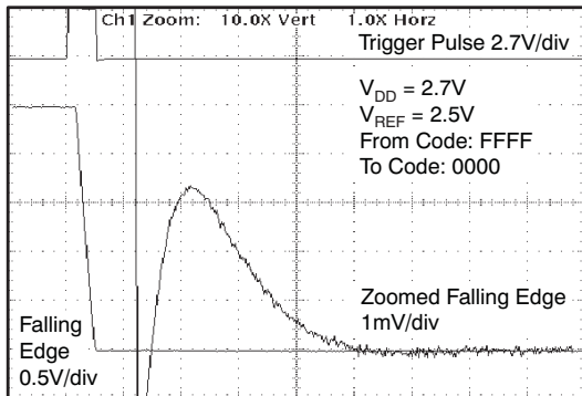
Figure 37. Full-Scale Settling Time: Falling Edge
