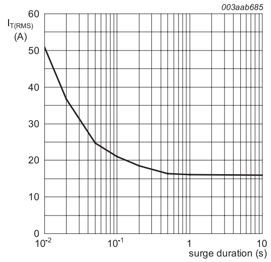
f = 50 Hz; T_{mb} = 101 °C Fig. 3. RMS on-state current as a function of surge duration; maximum values
